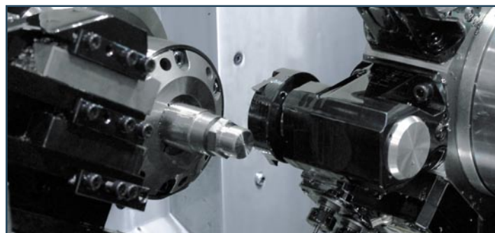
Polygon Machining on Miyano BNA
