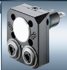
Twin Spindle X-axis [radial] Live Tool
